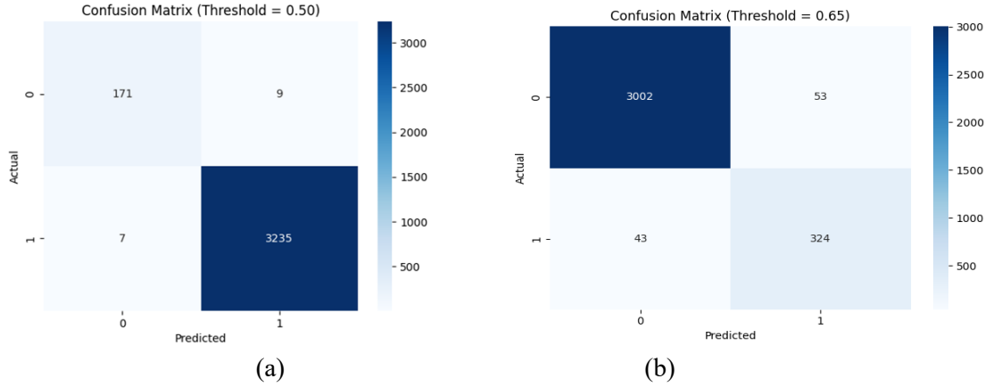
Figure 2: Confusion Matrix of Random Forest (a) Pedestrian presence in the crossing area (b) Legal or illegal pedestrian crossing
