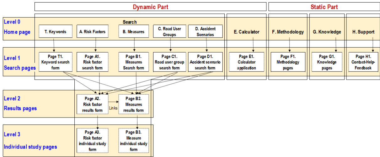
Figure 4: Overview of the Main Menu and entry points of the DSS.
