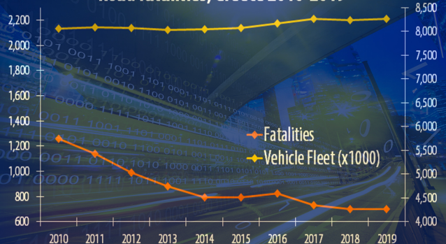
Road fatalities, Greece 2010-2019
